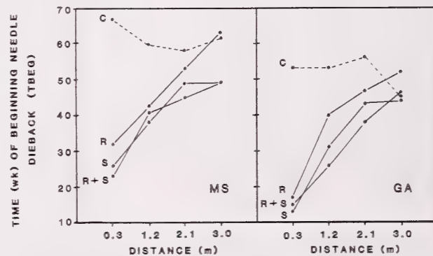
Figure 5.--Time (wk) of beginning brown spot needle dieback (TBEG) by distance (m) from initial infection focus for resistant (R), susceptible (S), mixed family (R+S), and control (C) plantings of longleaf pine in Mississippi (MS) and Georgia (GA).
